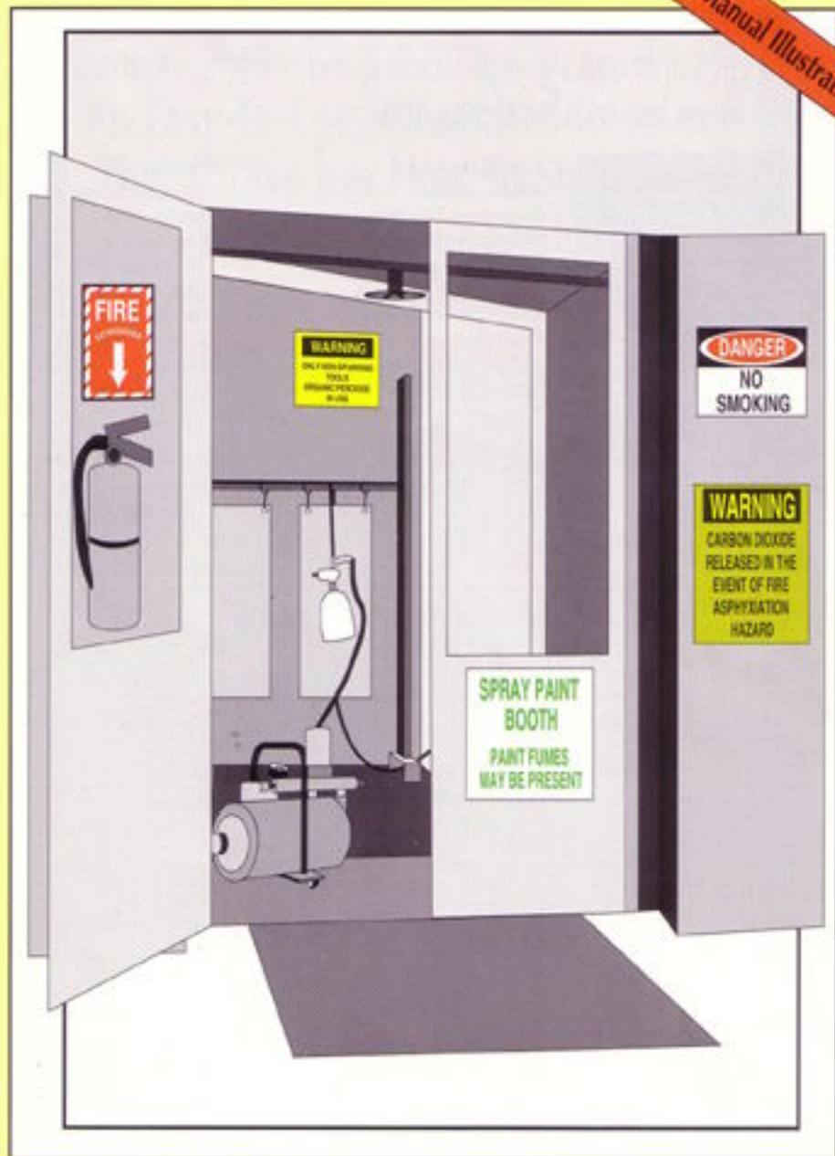
Spray paint area with required OSHA warning and informational signs for: no smoking, carbon dioxide, non-sparking tools, and paint fumes.
